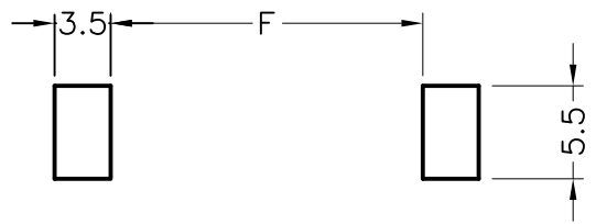
MOUNTING HOLES
