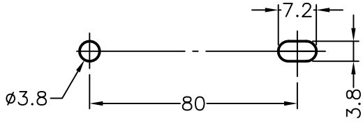
MOUNTING HOLES CHASSIS THICKNESS 1.6
