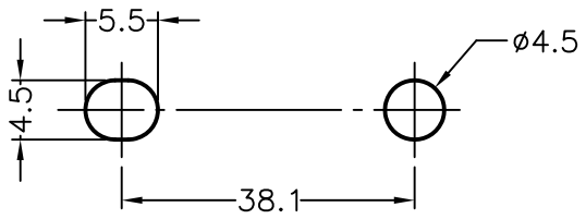
MOUNTING HOLES CHASSIS THICKNESS:0.8mm
