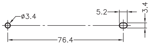
MOUNTION HOLE
