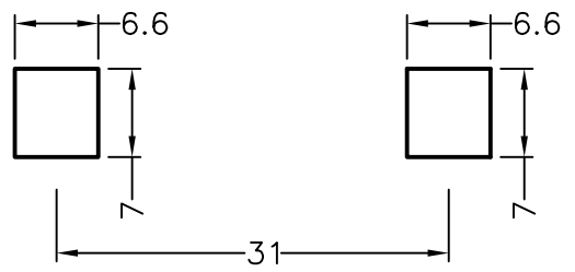
MOUNTING HOLES
