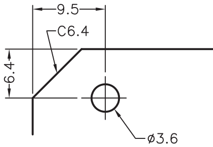
MOUNTING HOLE
