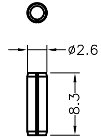
PIN
