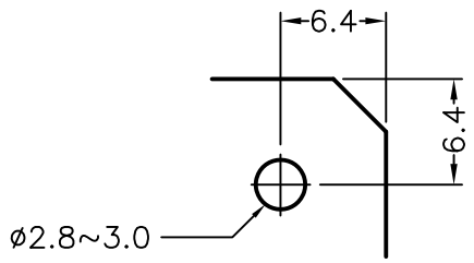
MOUNTING HOLE
