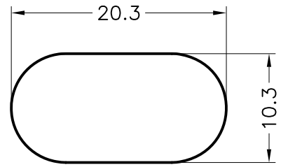
MOUNTING HOLE
