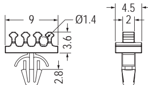
MOUNTING HOLE Ø2.5 THICKNESS 1.6
