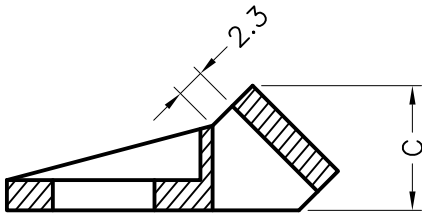
SECTION A-A Mounting Screw Size 5/16
