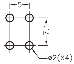
MOUNTING HOLE
