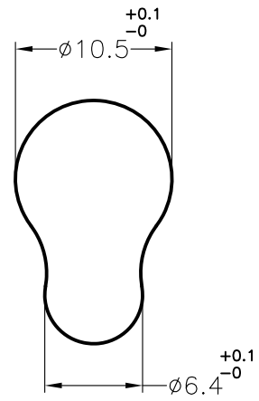
MOUNTING HOLE
