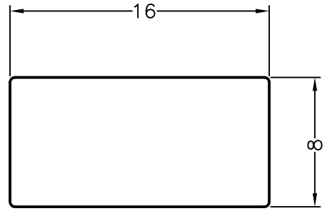
MOUNTING HOLE
