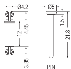
MOUNTING HOLE Ø3.3 THICKNESS 1.6
