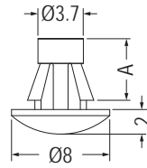
MOUNTING HOLE Ø4.0 THICKNESS 0.8-1.6
