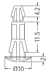
MOUNTING HOLE Ø5.5 THICKNESS 1.5-2.2
