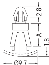
MOUNTING HOLE Ø4.8 THICKNESS 0.8-2.0
