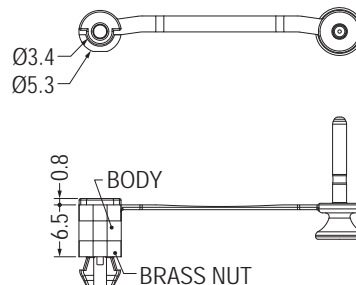
MOUNTING HOLE THICKNESS 1.6
