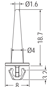
MOUNTING HOLE Ø4.6 THICKNESS 1.3
