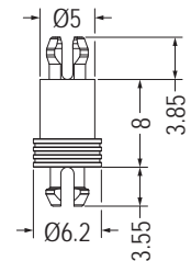
MOUNTING HOLE Ø3.2 THICKNESS 1.8
