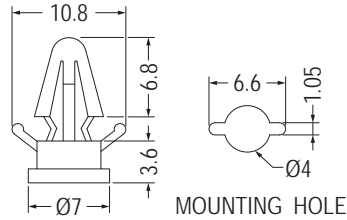
THICKNESS 1.2-1.7
