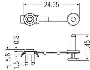
MOUNTING HOLE Ø4.0 THICKNESS 2.3-2.9
