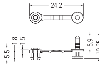
MOUNTING HOLE Ø4.0 THICKNESS 1.6
