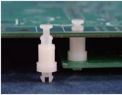
MOUNTING HOLE Ø3.3 THICKNESS 1.57
