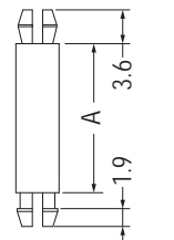
MOUNTING HOLE Ø3.9 THICKNESS 1.6
