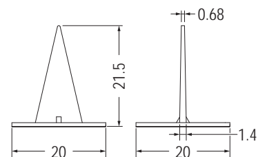
DOUBLE ADHESIVE TAPE
