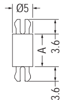
MOUNTING HOLE Ø3.3 THICKNESS 1.6
