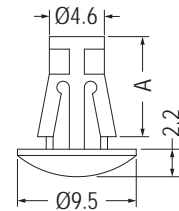
MOUNTING HOLE Ø4.8 THICKNESS 0.8-1.2
