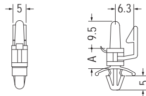
MOUNTING HOLE Ø4.8 THICKNESS 0.5-2.0
