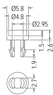
MOUNTING HOLE Ø4.0 THICKNESS 2.3-2.5
