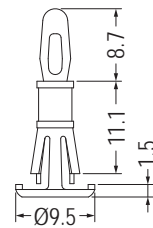
MOUNTING HOLE Ø4.8 THICKNESS 1.5-1.6
