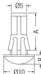
MOUNTING HOLE Ø5.5 THICKNESS 1.6-2.5
