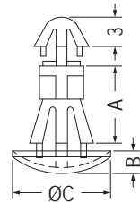
MOUNTING HOLE Ø5.0 THICKNESS 0.8-1.8
