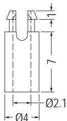
FOR M2 SCREW
