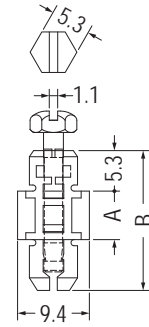
MOUNTING HOLE \varnothing 6.4\text{-}\varnothing 6.5 THICKNESS 0.8-1.6
