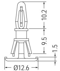
MOUNTING HOLE Ø6.35 THICKNESS 1.0-1.6
