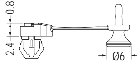
MOUNTING HOLE THICKNESS 1.6-2.1 3.2
