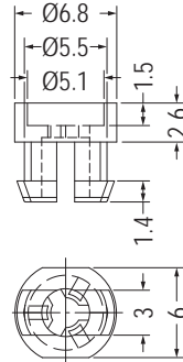
MOUNTING HOLE Ø5.5 THICKNESS 2.3-2.5
