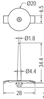
MOUNTING HOLE Ø5.0 THICKNESS 0.75-1.05
