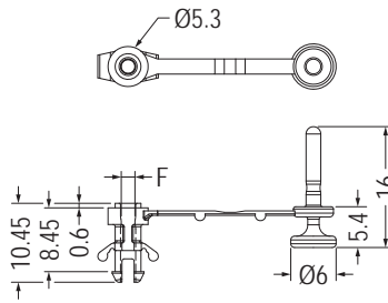
MOUNTING HOLE Ø3.5 THICKNESS 1.6-2.2
