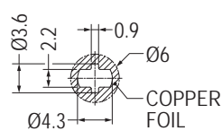
MOUNTING HOLE THICKNESS 1.6
