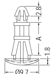
MOUNTING HOLE Ø4.8 THICKNESS 0.8-2.0
