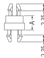
MOUNTING HOLE Ø4.8 THICKNESS 1.6
