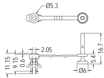
MOUNTING HOLE Ø3.5 THICKNESS 2.3-2.9
