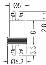
MOUNTING HOLE Ø3.2 THICKNESS 1.72
