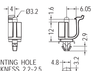
THICKNESS 1.6
