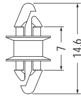
MOUNTING HOLE \varnothing 4.0 THICKNESS 1.6-1.9
