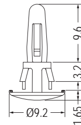
MOUNTING HOLE Ø4.8 THICKNESS 1.7
