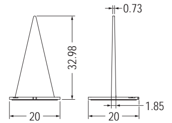
DOUBLE ADHESIVE TAPE
