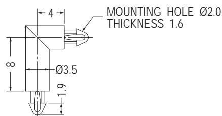
MOUNTING HOLE \varnothing 2.0 THICKNESS 1.6
