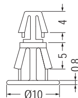
MOUNTING HOLE Ø5.5 THICKNESS 1.5-2.2
