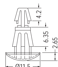
MOUNTING HOLE Ø5.5 THICKNESS 2.0-3.0
