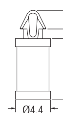
MOUNTING HOLE Ø2.5 THICKNESS 1.0
