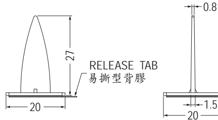
DOUBLE ADHESIVE TAPE
