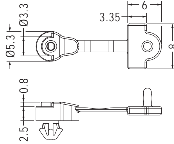
MOUNTING HOLE Ø3.0 THICKNESS 1.2
