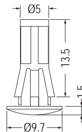
MOUNTING HOLE Ø5.5 THICKNESS 1.2-1.8
