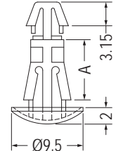
MOUNTING HOLE Ø4.8 THICKNESS 0.8-1.2
