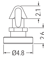
MOUNTING HOLE Ø2.0 THICKNESS 1.4
