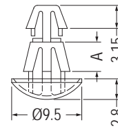
MOUNTING HOLE Ø4.8 THICKNESS 0.8-1.2
