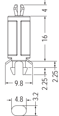
MOUNTING HOLE THICKNESS 1.8-2.0
