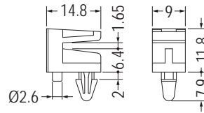
MOUNTING HOLE THICKNESS 1.6
