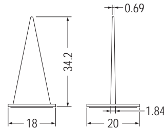
WHITE REFLECTING SHEET
