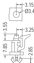
MOUNTING HOLE Ø3.4 THICKNESS 1.2
