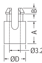
FOR M3 SCREW
