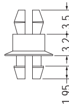
MOUNTING HOLE Ø3.9 THICKNESS 1.6
