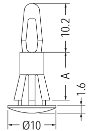
MOUNTING HOLE Ø5.5 THICKNESS 1.0-1.7
