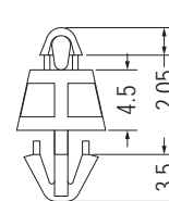
MOUNTING HOLE Ø4.0 THICKNESS 1.6
