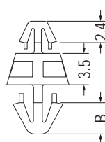
MOUNTING HOLE Ø4.0 THICKNESS: T
