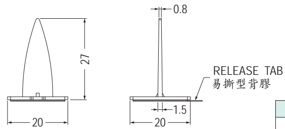
DOUBLE ADHESIVE TAPE
