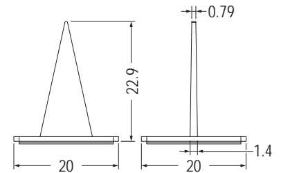
WHITE REFLECTING SHEET
