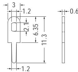
MOUNTING HOLE Ø1.2-Ø1.3
