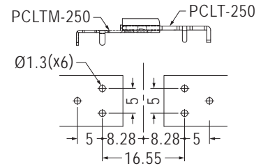
COMBINATION ILLUSTRATION DWG MOUNTING HOLE
