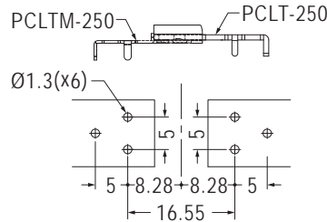
COMBINATION ILLUSTRATION DWG MOUNTING HOLE
