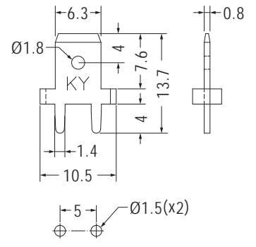
MOUNTING HOLE
