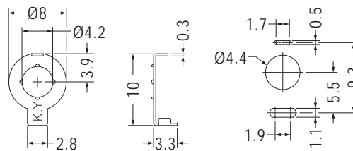
MOUNTING HOLE
