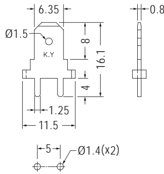
MOUNTING HOLE
