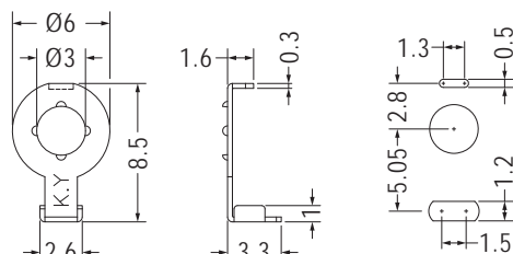
MOUNTING HOLE
