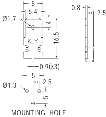
COMBINATION ILLUSTRATION DWG MOUNTING HOLE
