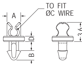
MOUNTING HOLE: \varnothing 2.0 THICKNESS: T
