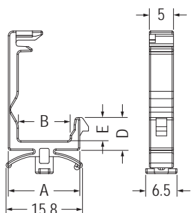
MOUNTING HOLE THICKNESS 0.8-1.6
