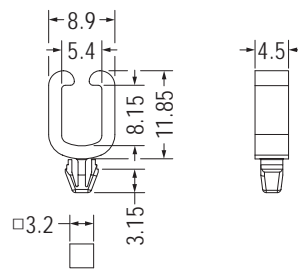
MOUNTING HOLE THICKNESS 0.6-1.2
