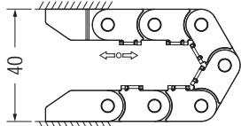
PRINCIPLE SKETCH - BEND RA-DIUS
