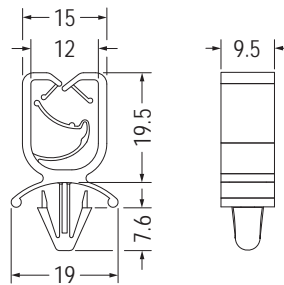
MOUNTING HOLE Ø6.3~Ø7.0 THICKNESS 0.6~3.0
