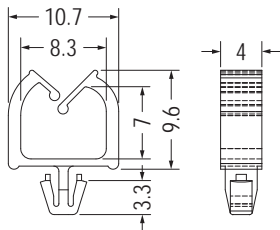
MOUNTING HOLE Ø3.3 THICKNESS 1.0
