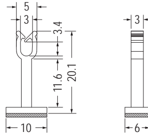
3M DOUBLE ADHESIVE TAPE THICKNESS 0.9
