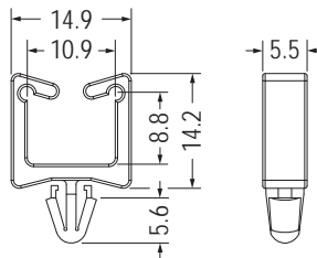
MOUNTING HOLE Ø4.8 THICKNESS 1.1
