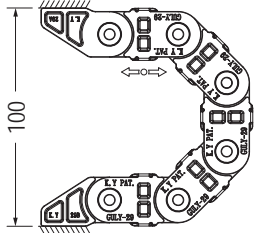
PRINCIPLE SKETCH - BEND RA-DIUS
