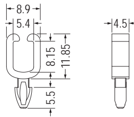
MOUNTING HOLE \varnothing 4.0 THICKNESS 2.2
