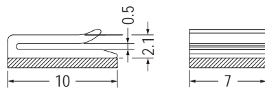
3M DOUBLE ADHESIVE TAPE
