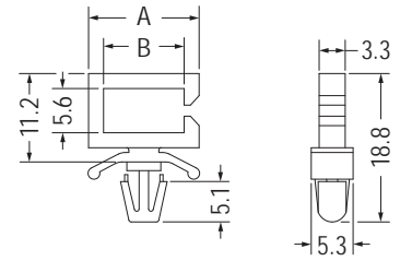
MOUNTING HOLE Ø4.8 THICKNESS 0.8-2.0
