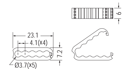
UNIT FOLDED VIEW
