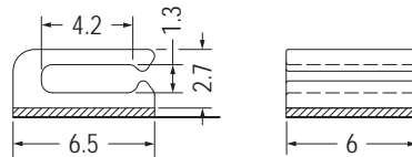
3M DOUBLE ADHESIVE TAPE WITH RELEASE TAB 易撕型背膠
