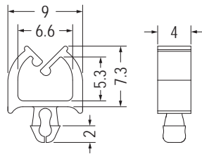
MOUNTING HOLE Ø3.0 THICKNESS 1.2~1.6
