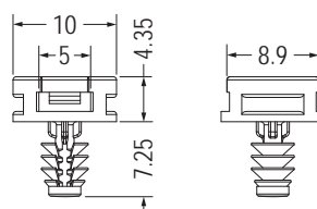
MOUNTING HOLE \varnothing 3.3\text{-}\varnothing 4.0 (M4) THICKNESS 1.0-3.0
