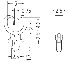
MOUNTING HOLE Ø2.0 THICKNESS 1.6
