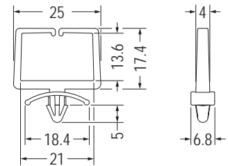
MOUNTING HOLE \varnothing 4.8-\varnothing 5.0 THICKNESS 0.8-2.5
