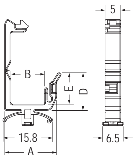
MOUNTING HOLE THICKNESS 0.8-1.6
