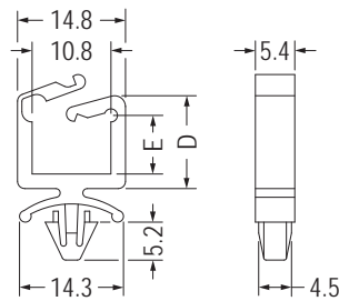
MOUNTING HOLE Ø4.8~Ø5.0 THICKNESS 0.5~2.0
