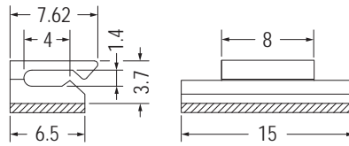
3M DOUBLE ADHESIVE TAPE
