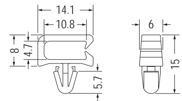
MOUNTING HOLE Ø4.8 THICKNESS 0.8-1.6
