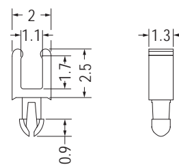
MOUNTING HOLE \varnothing 1.0 THICKNESS 1.0
