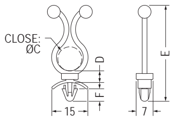
MOUNTING HOLE Ø4.8-Ø5.0 THICKNESS 0.8-2.0
