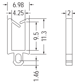
MOUNTING HOLE Ø2.8 THICKNESS 2.0
