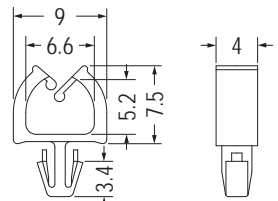
MOUNTING HOLE Ø3.0 THICKNESS 1.6
