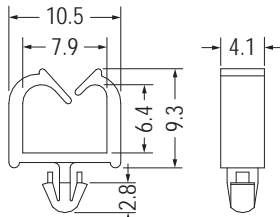
MOUNTING HOLE Ø3.0 THICKNESS 0.8-1.6
