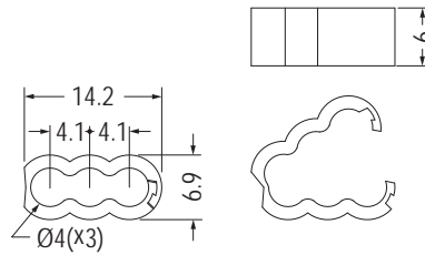
UNIT FOLDED VIEW
