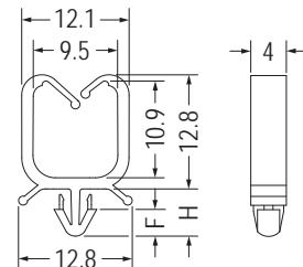
MOUNTING HOLE: ØG THICKNESS 0.6-1.6
