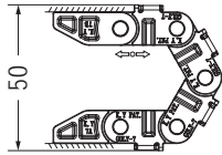
PRINCIPLE SKETCH - BEND RA-DIUS
