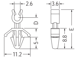
MOUNTING HOLE Ø4.0 THICKNESS 0.8-2.5
