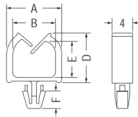
MOUNTING HOLE: ØG THICKNESS: T
