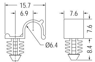
MOUNTING HOLE Ø6.35 THICKNESS 6.35
