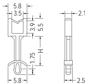
MOUNTING HOLE Ø2.0 THICKNESS 1.6-1.8
