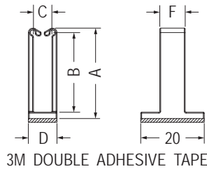
3M DOUBLE ADHESIVE TAPE
