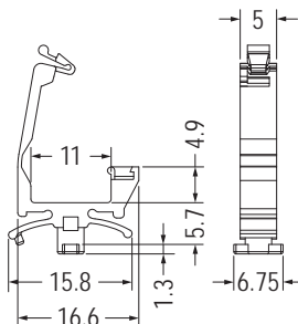
MOUNTING HOLE THICKNESS 0.8-2.0
