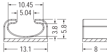
3M DOUBLE ADHESIVE TAPE
