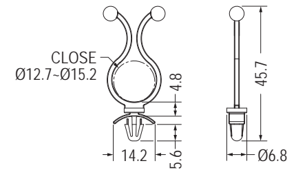
MOUNTING HOLE Ø4.75-Ø4.8 THICKNESS 0.8-2.0
