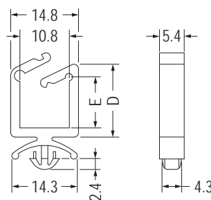
MOUNTING HOLE Ø4.8 THICKNESS 0.8~1.6
