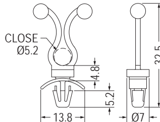
MOUNTING HOLE Ø4.8 THICKNESS 0.8-2.0
