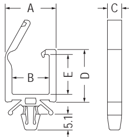
MOUNTING HOLE Ø4.8 THICKNESS 0.5-2.0
