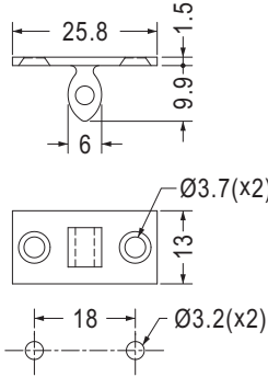
MOUNTING HOLE
