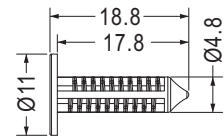
MOUNTING HOLE Ø5.0 THICKNESS 1.5~11.0
