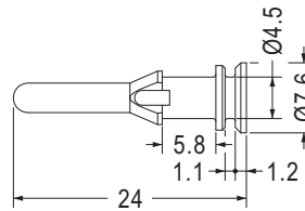
MOUNTING HOLE Ø4.5 THICKNESS 0.8~1.0
