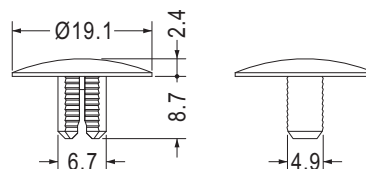
MOUNTING HOLE \varnothing 7.1 ASSEMBLED THICKNESS 8.8~12.8
