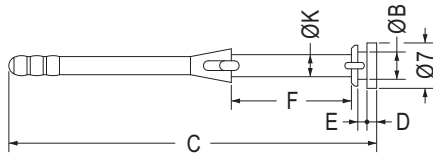
MOUNTING HOLE: ØG THICKNESS: E
