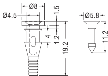
MOUNTING HOLE Ø4.5
