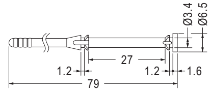
MOUNTING HOLE Ø3.7 THICKNESS 1.0~1.2
