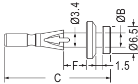
MOUNTING HOLE: ØG THICKNESS 1.5~1.6
