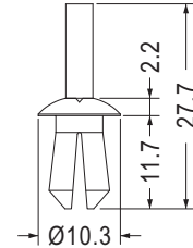
MOUNTING HOLE Ø6.0 THICKNESS 6.0
