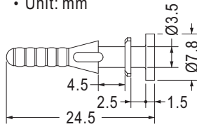
MOUNTING HOLE Ø3.5 THICKNESS 2.5
