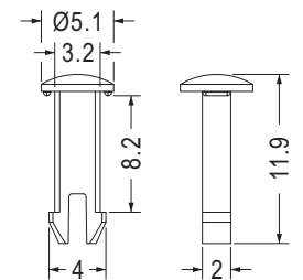
MOUNTING HOLE Ø3.3 THICKNESS 7.7
