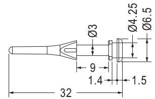
MOUNTING HOLE Ø4.4 THICKNESS 1.2~1.6
