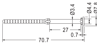
MOUNTING HOLE Ø4.5 THICKNESS 0.8~1.0
