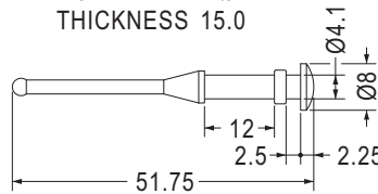
MOUNTING HOLE Ø4.4 THICKNESS 2.4~2.6
