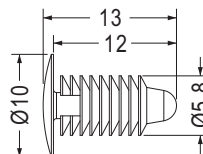
MOUNTING HOLE Ø5.5 THICKNESS 0.7~6.4
