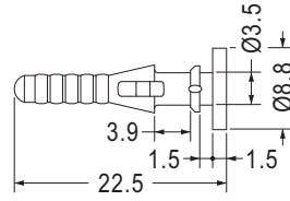
MOUNTING HOLE Ø3.5 THICKNESS 1.4~1.6
