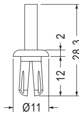
MOUNTING HOLE Ø6.4 THICKNESS 4.0~9.5
