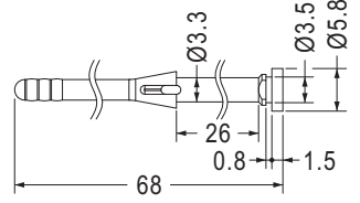
MOUNTING HOLE Ø3.4 THICKNESS 0.8~1.0
