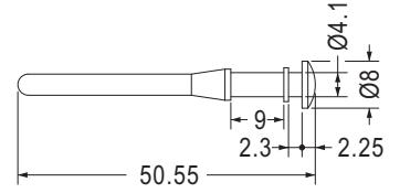
MOUNTING HOLE Ø4.3 THICKNESS 2.2~2.4
