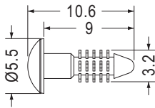
MOUNTING HOLE Ø3.0
