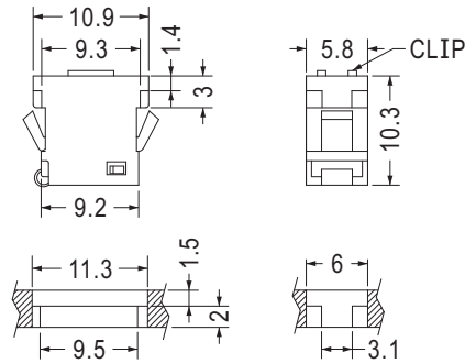
MOUNTING HOLE
