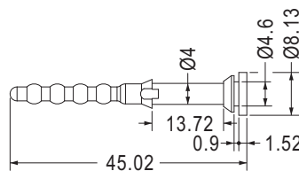
MOUNTING HOLE Ø5.5 THICKNESS 0.8~1.0
