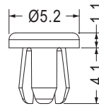
MOUNTING HOLE \varnothing 3.2 THICKNESS 0.8~2.4
