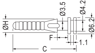
MOUNTING HOLE Ø3.5 THICKNESS 1.1~1.2
