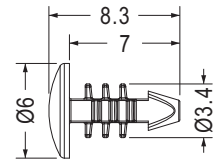
MOUNTING HOLE Ø2.7~3.3 THICKNESS 1.5~4.0
