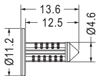
MOUNTING HOLE Ø5.0 THICKNESS 2.5~4.5
