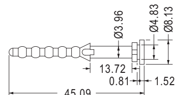
MOUNTING HOLE Ø5.1 THICKNESS 0.8~1.0
