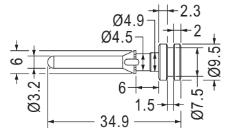
MOUNTING HOLE Ø7.5 THICKNESS 1.5~1.6
