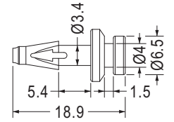
MOUNTING HOLE Ø4.0 THICKNESS 1.5~1.6
