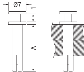
MOUNTING HOLE Ø4.0 THICKNESS: T
