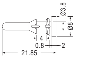
MOUNTING HOLE Ø4.4~Ø4.5 THICKNESS 0.8~1.0
