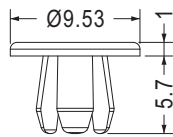
MOUNTING HOLE \varnothing 4.8 THICKNESS 0.8~3.6
