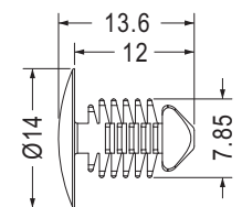
MOUNTING HOLE Ø7.0~Ø7.1 THICKNESS 3.0~7.0
