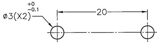
MOUNTING HOLES CHASSIS THICKNESS 1.6mm
