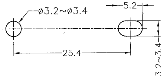
MOUNTING HOLE (RECOMMEND FOR REFERENCE ONLY)
