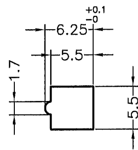
MOUNTING HOLE BOARD THICKNESS : 2.0~3.0mm
