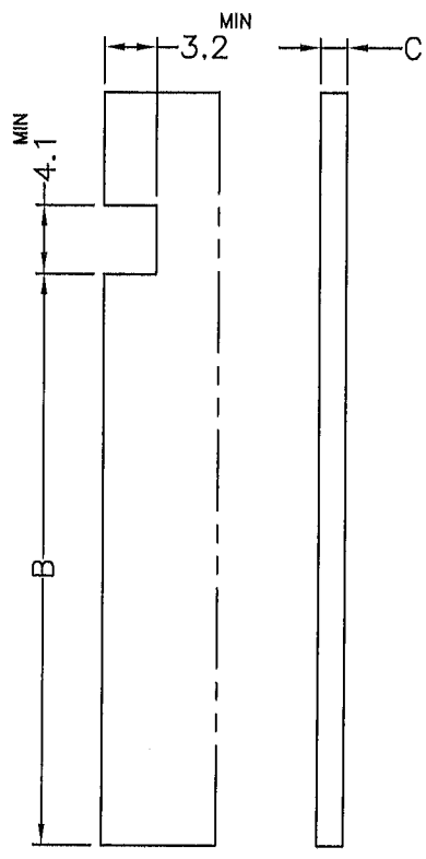
TYPICAL BOARD CUT-OUT
