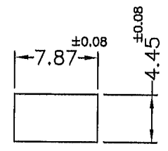
MOUNTING HOLE CHASSIS THICKNESS 0.76~1.78mm
