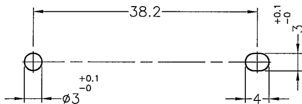
MOUNTING HOLE THICKNESS 1.6mm
