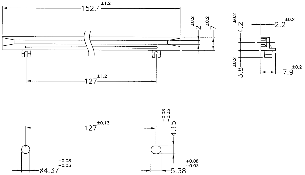
MOUNTING HOLE PANEL THICKNESS 1.2~2.3mm
