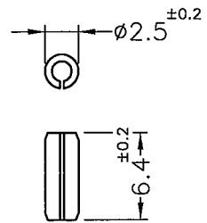
PIN
