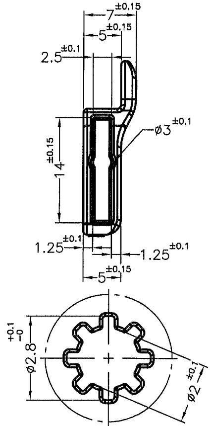
DETAIL A SCALE 4:1
