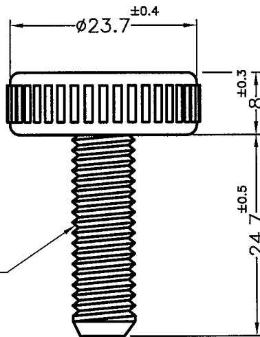
SCREW M8X1.25P (INSERT MOLDING)
