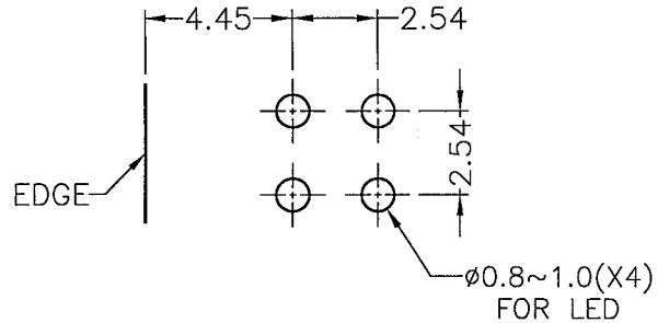
MOUNTING HOLE (RECOMMEND FOR REFERENCE ONLY)
