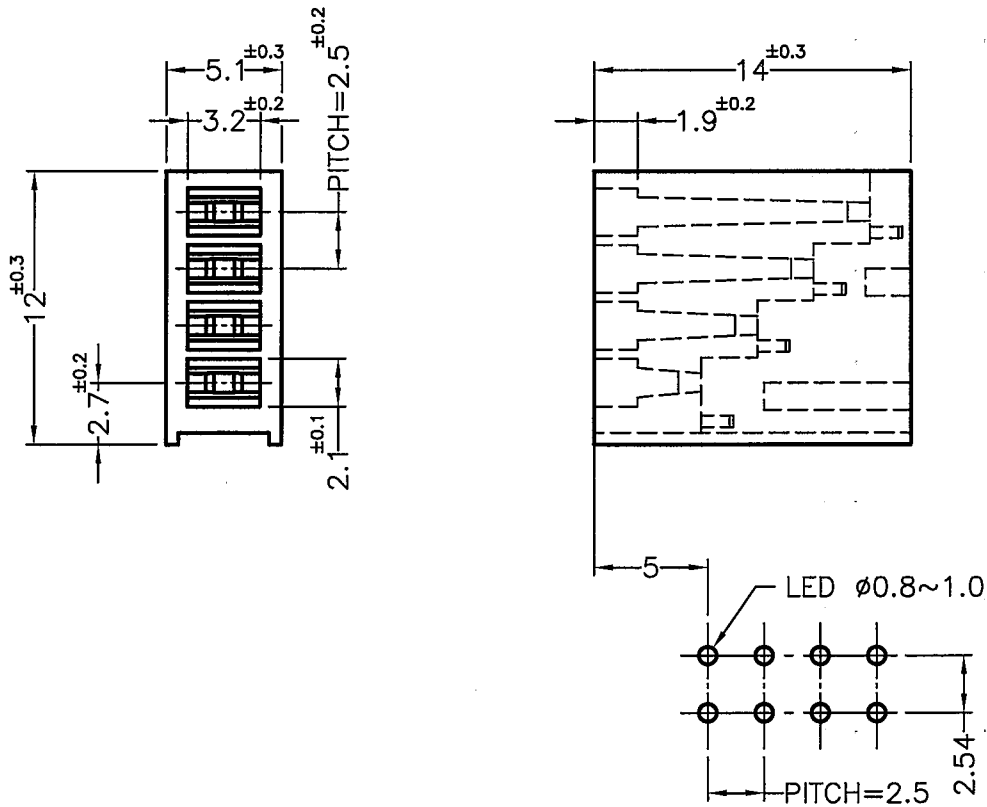
MOUNTING HOLE
