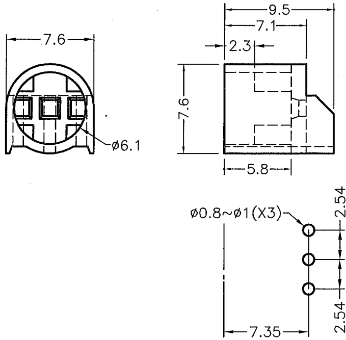
MOUNTING HOLE
