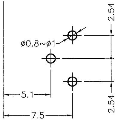
MOUNTING HOLE
