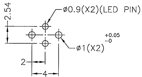
MOUNTING HOLE
