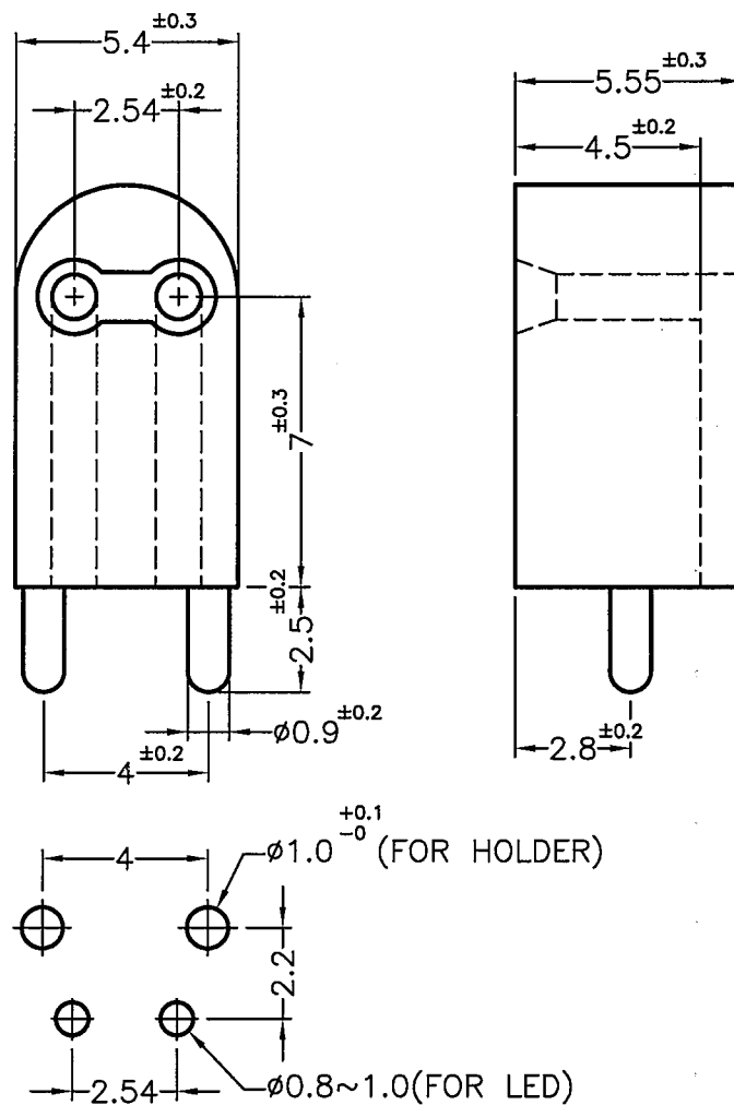
MOUNTING HOLE
