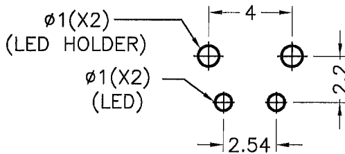
MOUNTING HOLES
