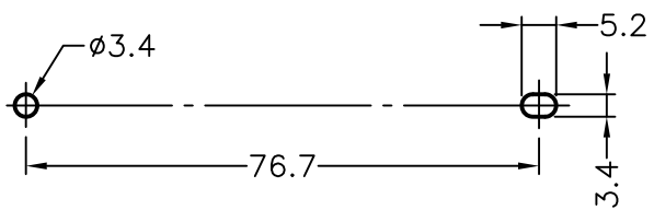
MOUNTING HOLE CHASSIS THICKNESS 1.2mm
