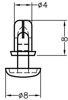
SNAP RIVET
