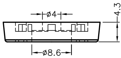
BODY
