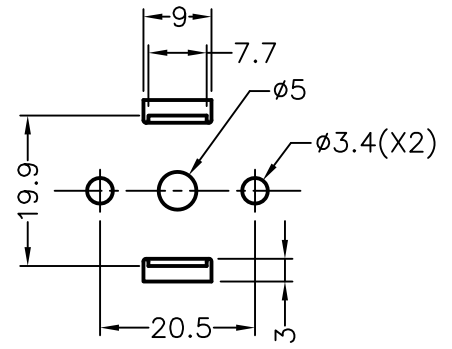
MOUNTING HOLES
