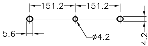
MOUNTING HOLES
