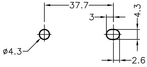
MOUNTING HOLES
