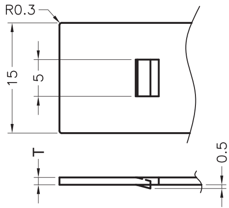
ASSEMBLY PART
