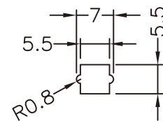
CHASSIS MOUNTING HOLE THICKNESS:0.8~1.2
