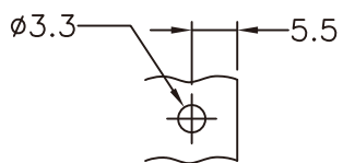
PCB MOUNTING HOLE THICKNESS:1.6
