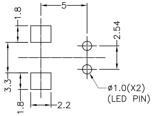
MOUNTING HOLES
