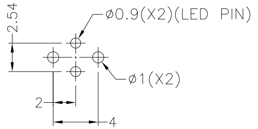
MOUNTING HOLES
