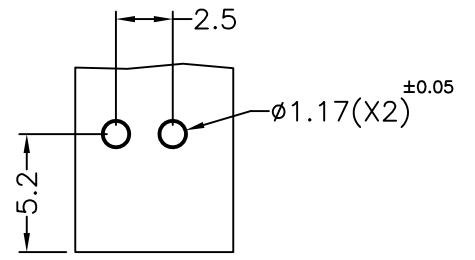
MOUNTING HOLE
