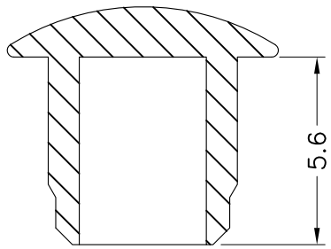
SECTION A-A MOUNTING HOLE \phi 5.5
