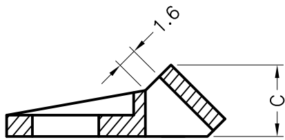
SECTION A-A Mounting Screw Size #10
