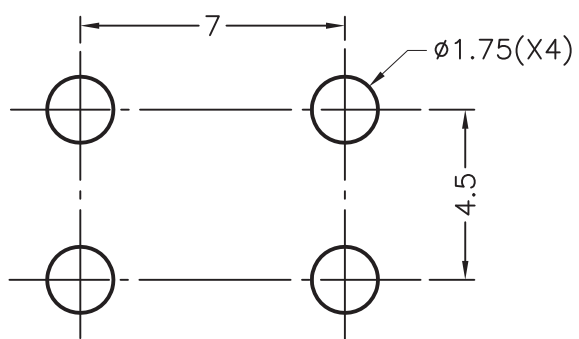
MOUNTING HOLE
