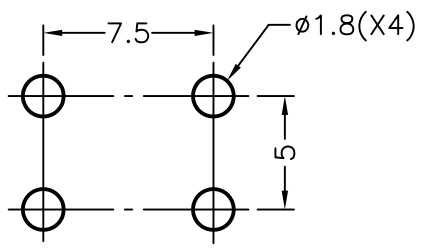
MOUNTING HOLES
