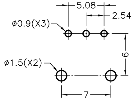
MOUNTING HOLES
