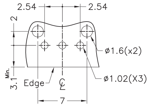
MOUNTING HOLE CHASSIS THICKNESS:1.6
