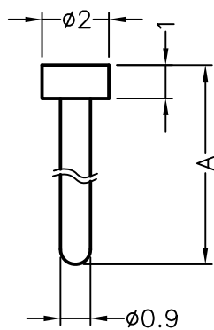
HOLE IN P.C BOARD \phi 0.9
